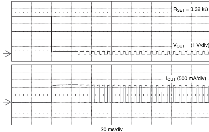
Figure 4. Current Over load Condition. Load Switch turned on with 0.1 \text{ }\Omega load at time = 0 ms.
