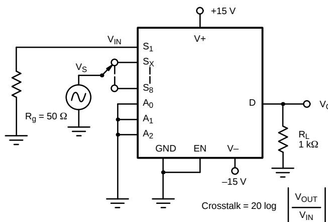
FIGURE 7. Crosstalk
