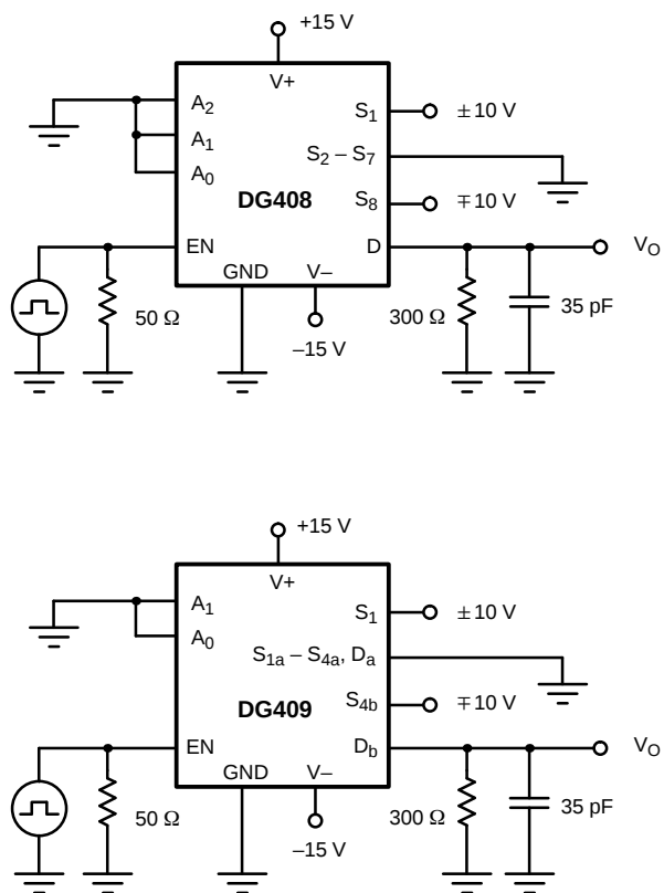
FIGURE 2. Transition Time
