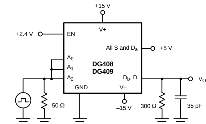
FIGURE 4. Break-Before-Make Interval
