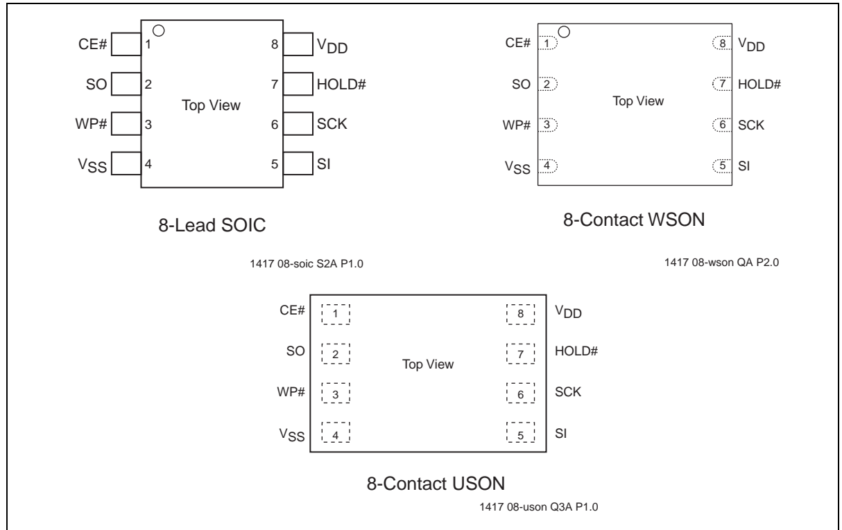
Figure 2: Pin Assignments
