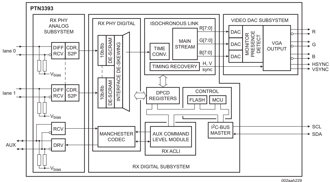
Fig 1. Functional diagram of PTN3393
