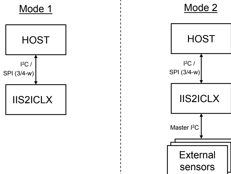
Figure 5. IIS2ICLX connection modes
