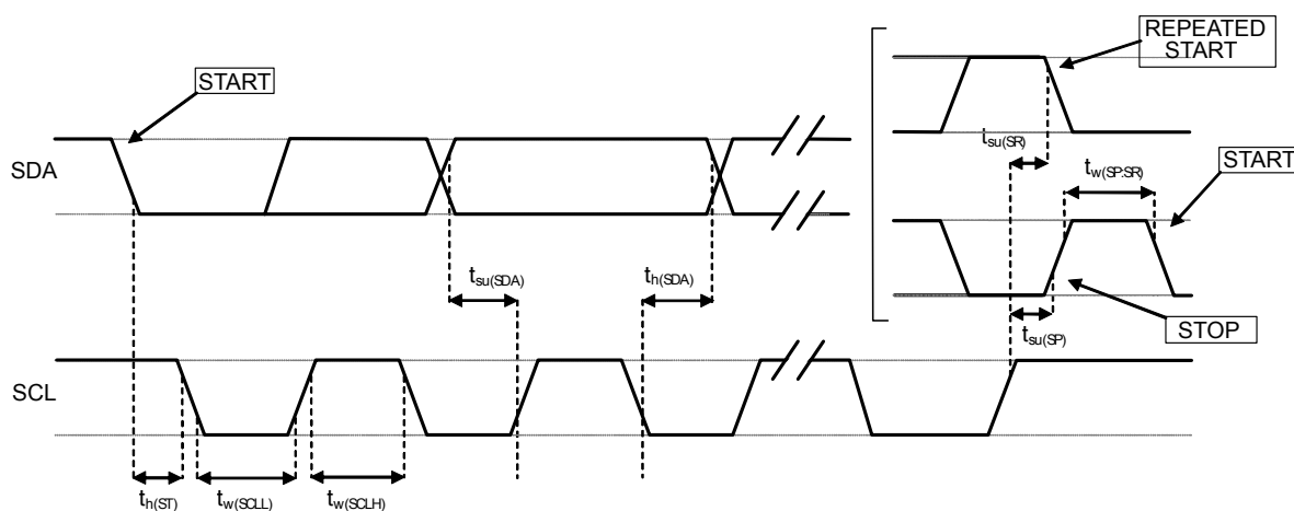
Figure 7. I 2 C slave timing diagram
