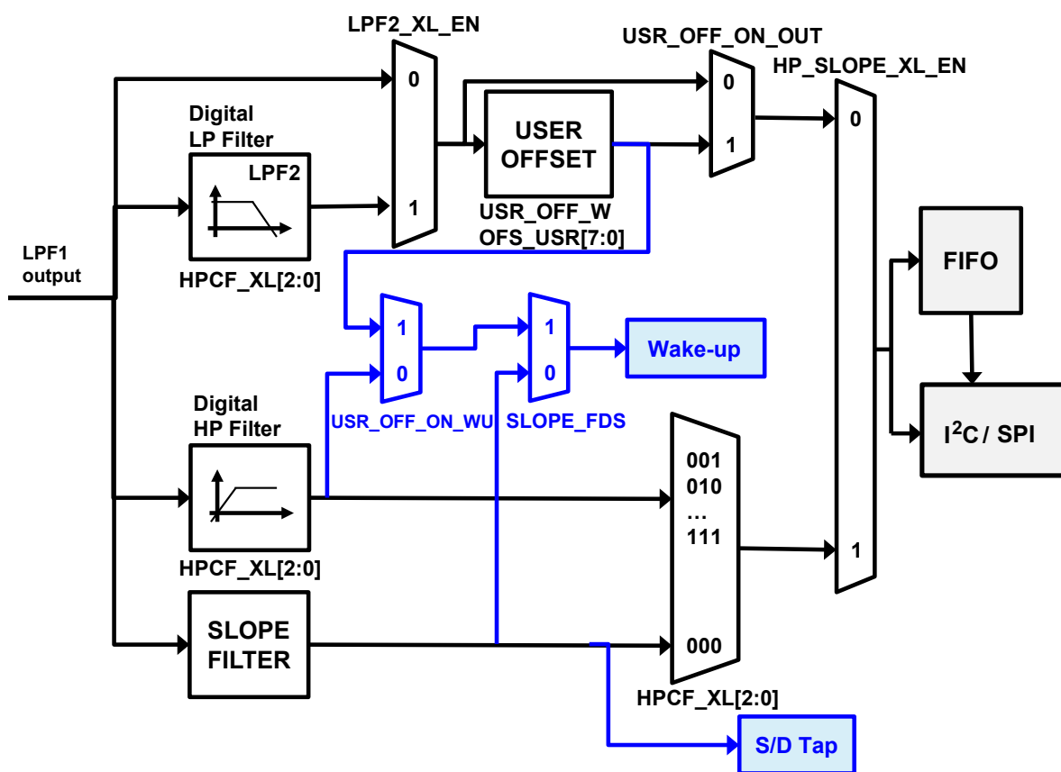
Figure 16. Accelerometer composite filter
