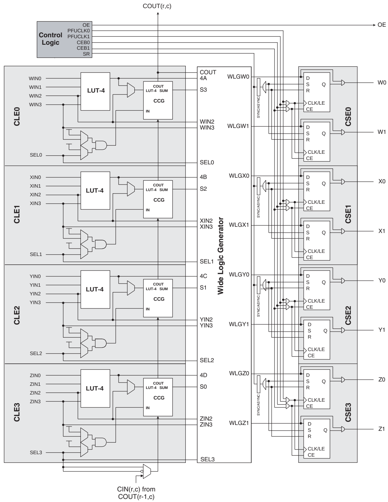
Figure 2. ispXPGA PFU
