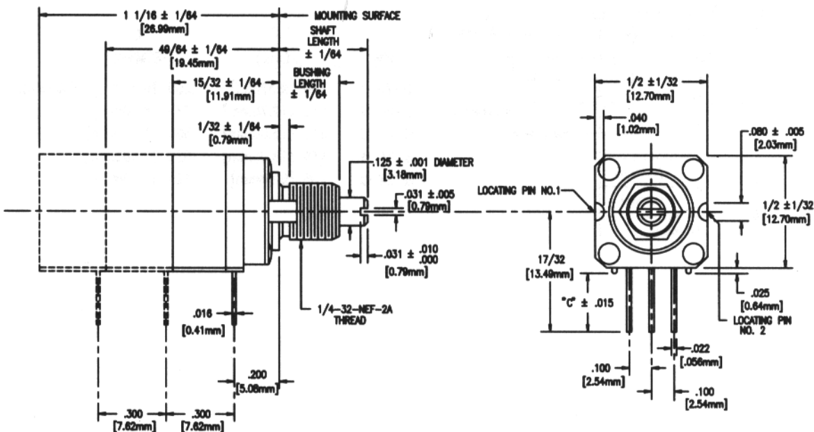
Figure 5 Series 408/409 Single, Dual or Triple (Second or Third Section May Be AL Series Rotary Switch) Printed Circuit - Type B-22 "C" Terminal Length: .875" (22.3mm) Maximum Standard PC Terminal Length: .250" (6.36mm)
