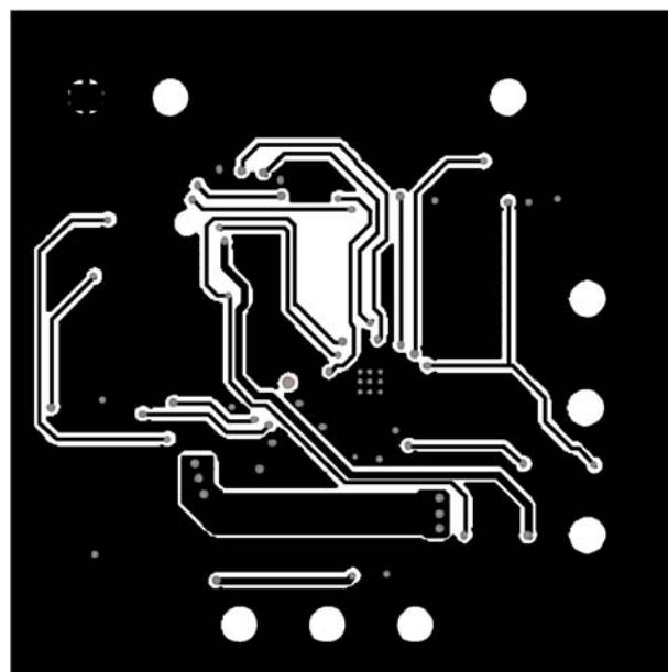
FIGURE 36. BOTTOM LAYER
