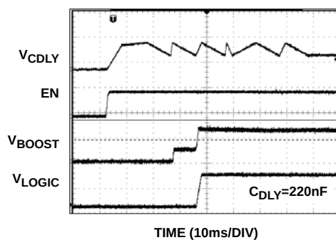
FIGURE 14. EL7586 START-UP SEQUENCE
