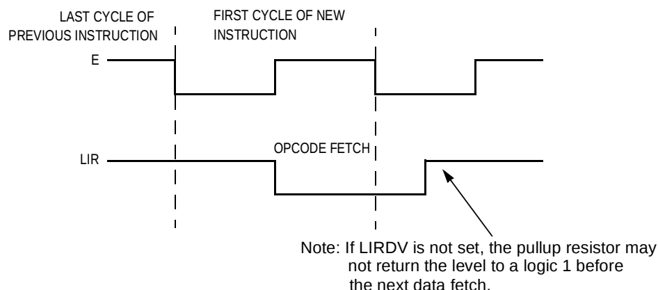
Figure 2-8. \overline{LIR} Timing
