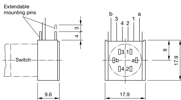
Component layout 1
