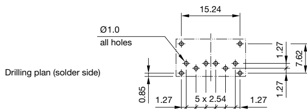
Component layout 3
