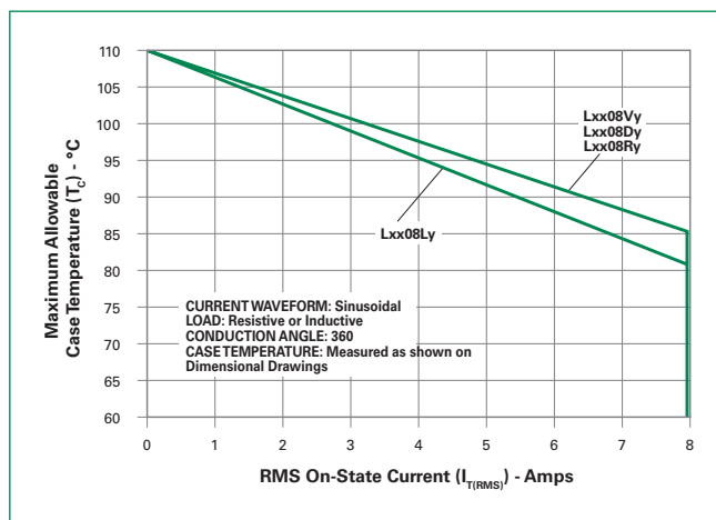
Figure 6: Maximum Allowable Case Temperature vs. On-State Current (Sensitive Triac)
