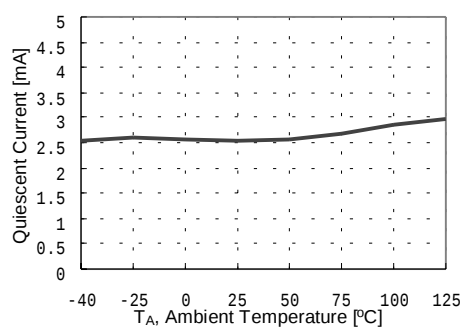
Figure 3. Quiescent Current
