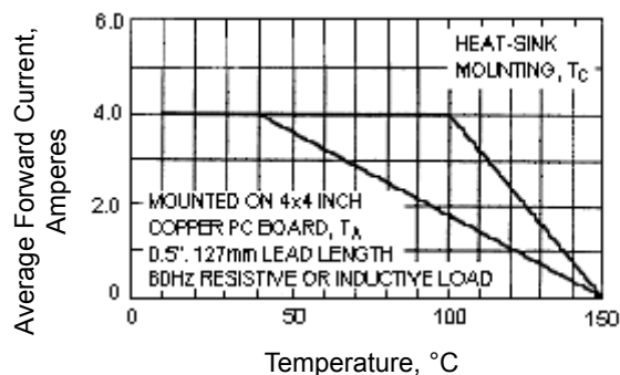
Figure - 1 Derating Curve for Output Rectified Current
