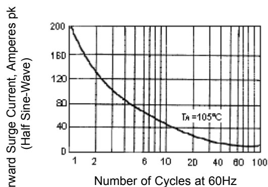
Figure - 4 Maximum Non-Repetitive Peak Forward Surge Current
