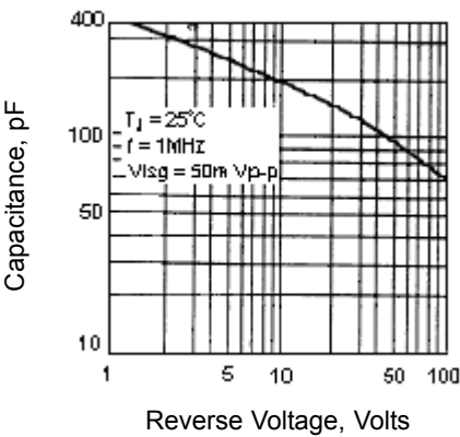
Figure - 5 Typical Junction Capacitance per Element
