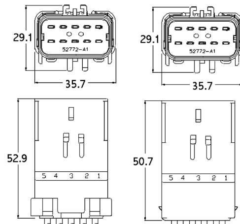
Sealed Assembly
