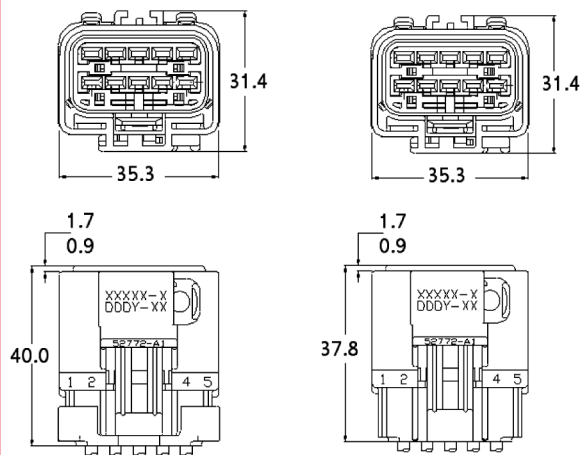
Sealed Assembly
