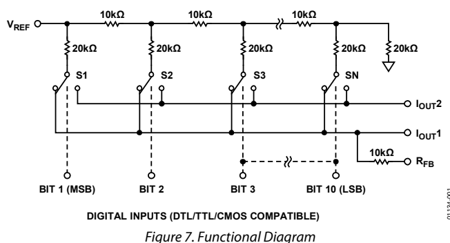
Figure 7. Functional Diagram
