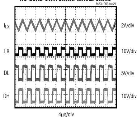
MAX1954/MAX1957 NO-LOAD SWITCHING WAVEFORMS
