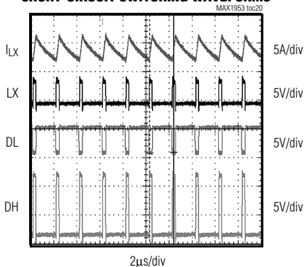
MAX1953 SHORT-CIRCUIT SWITCHING WAVEFORMS
