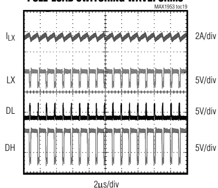
MAX1953 FULL-LOAD SWITCHING WAVEFORMS
