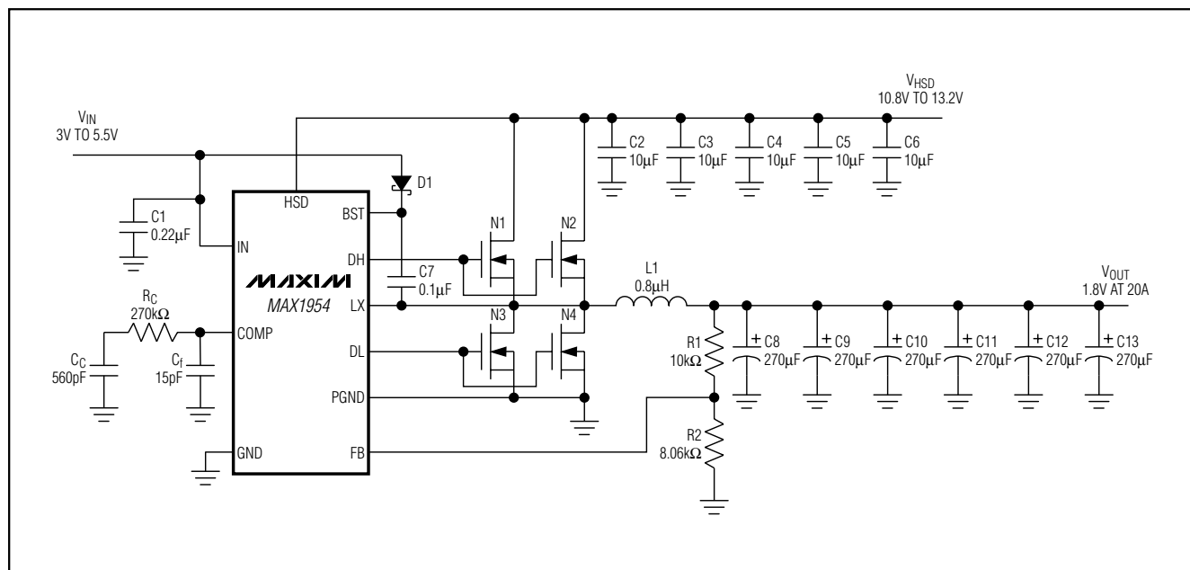
Figure 4. 20A Circuit
