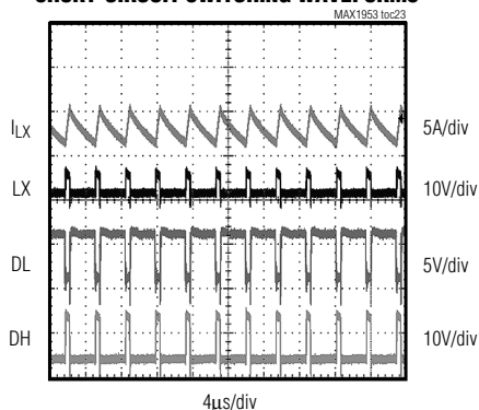
MAX1954/MAX1957 SHORT-CIRCUIT SWITCHING WAVEFORMS
