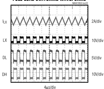
MAX1954/MAX1957 FULL-LOAD SWITCHING WAVEFORMS
