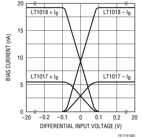
Bias Current vs Differential Input
