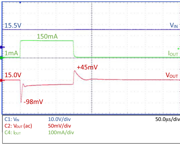
Figure 29. Load Transient – NCV8730–15.0 V, C_{OUT} = 22\text{ }\mu\text{F}
