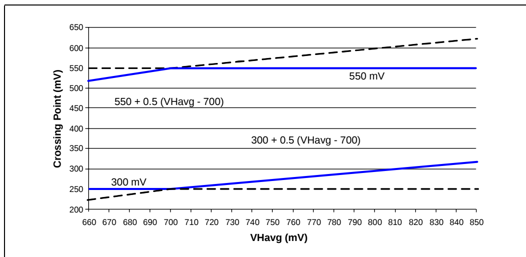
Figure 2-6. Differential Measurements
