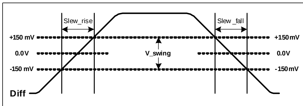
Figure 2-6. Differential Measurements
