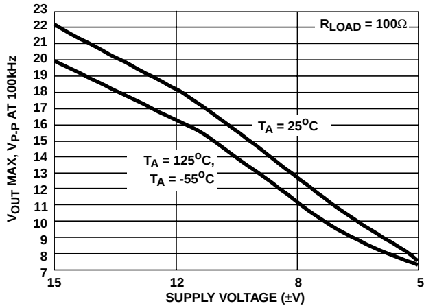
FIGURE 14. V_{\text{OUT}} MAXIMUM vs V_{\text{SUPPLY}}
