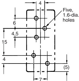
Mounting Holes
