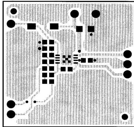
Figure 2–8. TPA321 EVM Top Layer
