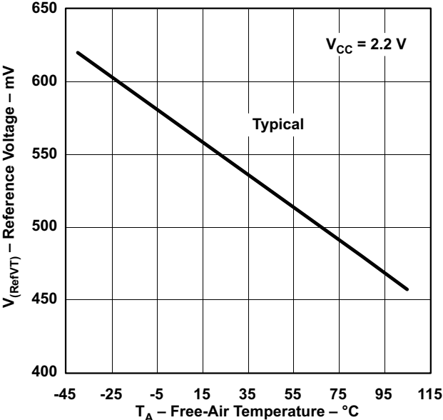
Figure 25. V_{(RefVT)} vs Temperature, V_{CC} = 2.2\text{ V}
