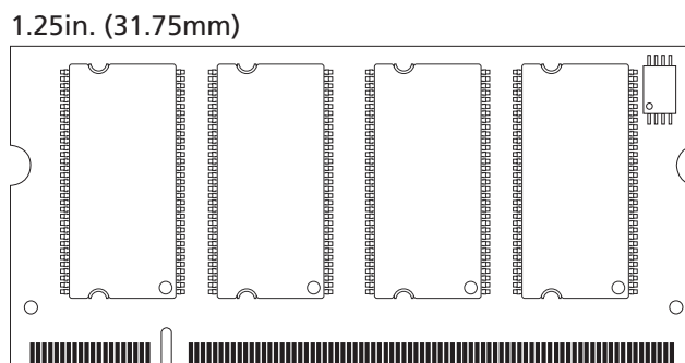
Figure 1: 200-Pin SODIMM (MO-224)
