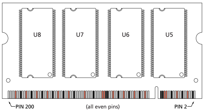
Figure 2: Module Layout
