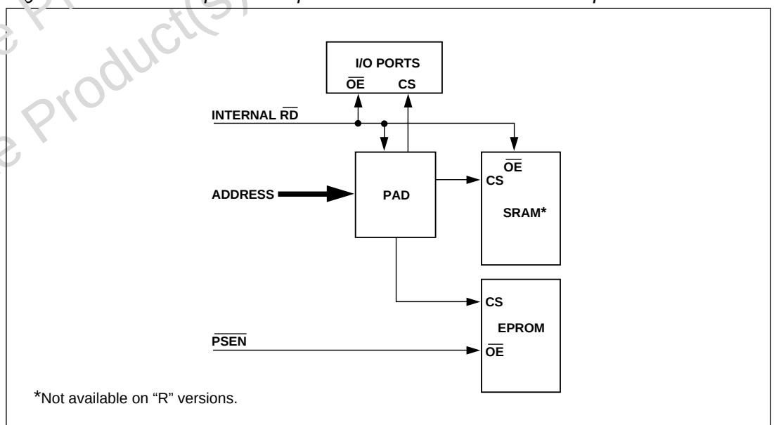
Figure 19. 8031-Compatible Separate Code and Data Address Spaces
