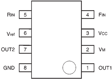
Fig.1 Pin assignments
