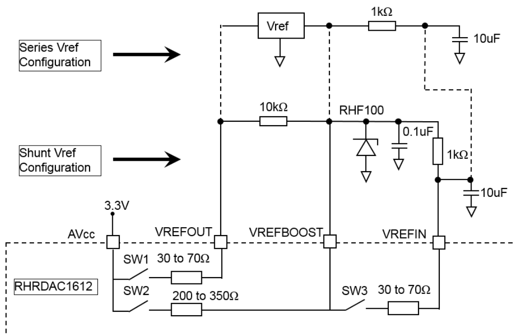
Figure 14. Internal switches for boost sequence
