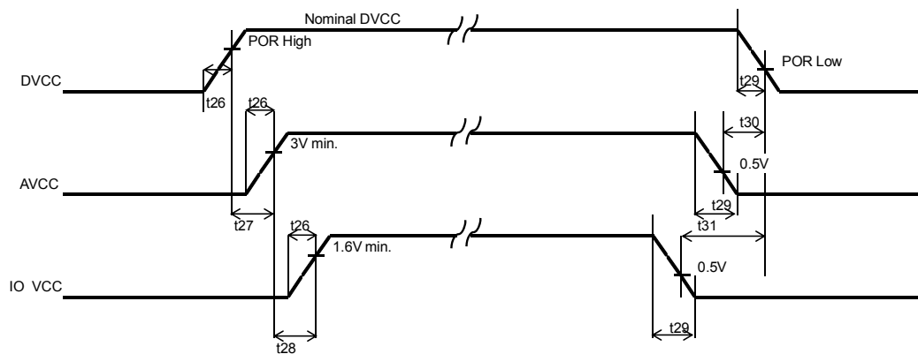
Figure 24. DAC timing diagram 3
