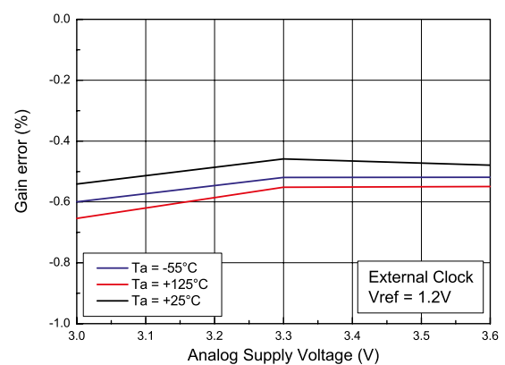
Figure 40. Gain error vs. AVCC vs. temperature, external master clock
