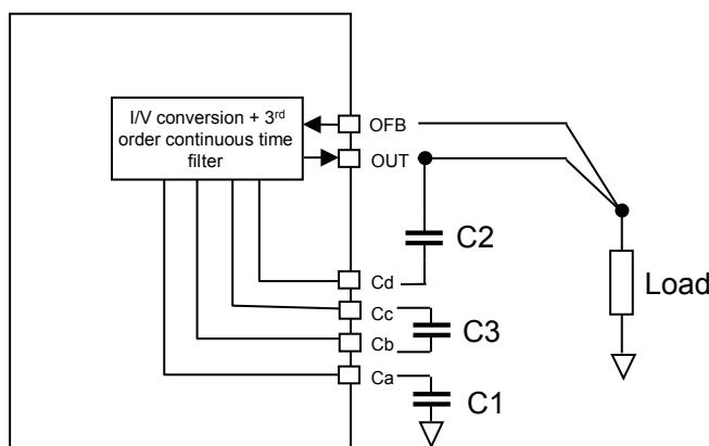
Figure 18. Another connection for C2
