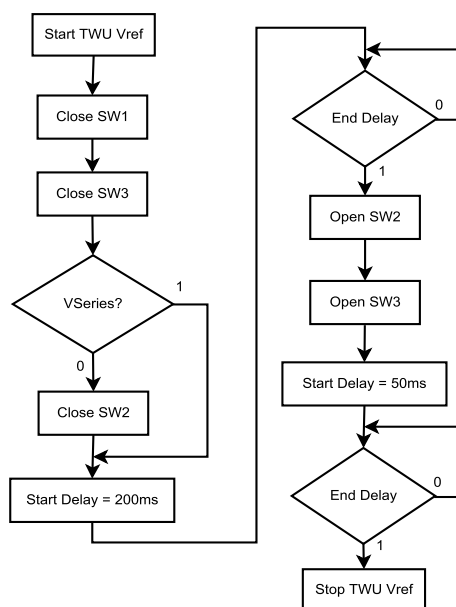
Figure 15. Boost sequence
