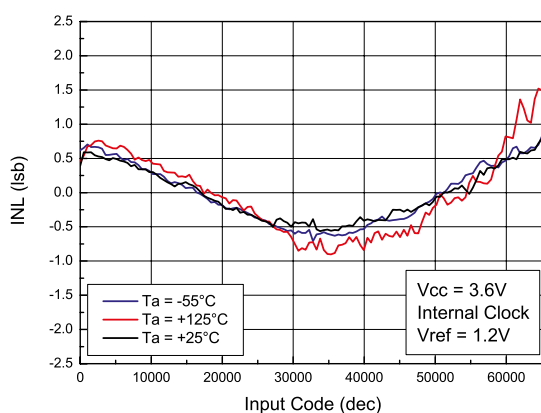
Figure 35. INL vs. input code vs. temperature, internal master clock, AVCC = 3.6 V
