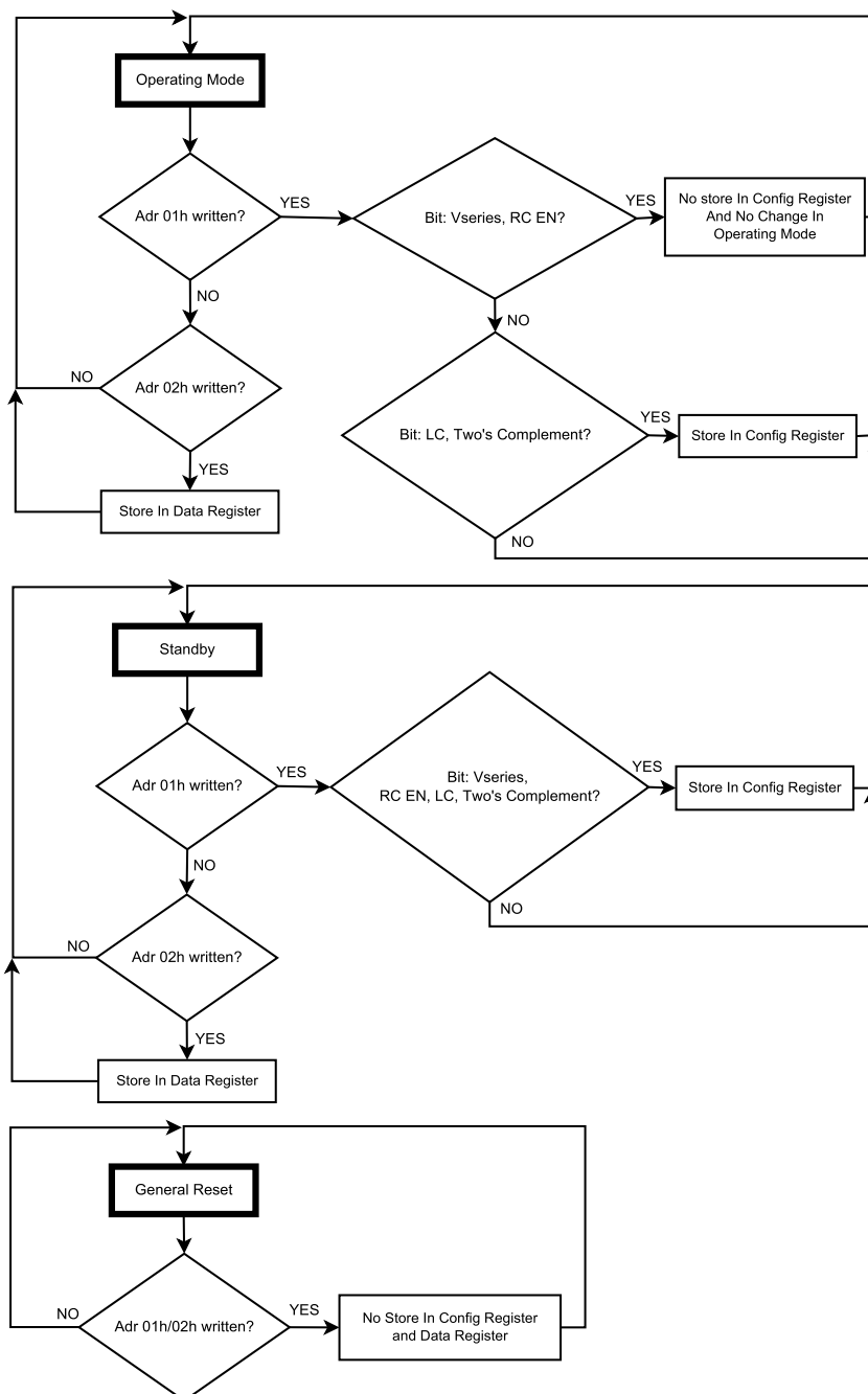
Figure 17. DAC operation flow chart (continued)
