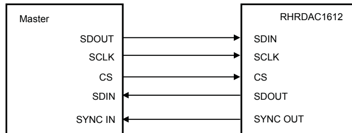
Figure 10. Connections between the DAC and the master
