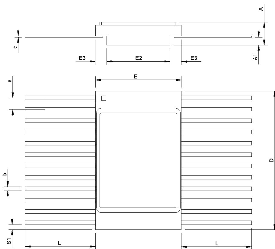
Figure 50. Ceramic Flat-24 package outline
