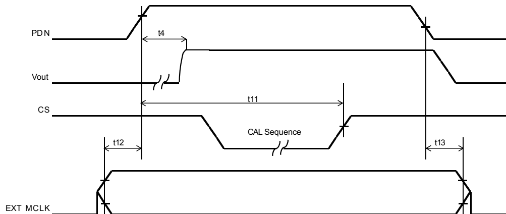
Figure 23. DAC timing diagram 2
