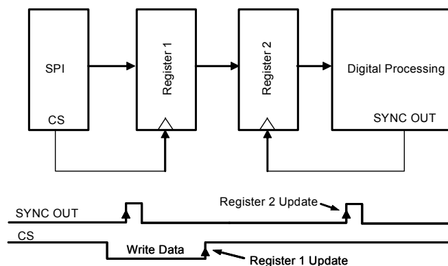
Figure 11. Asynchronous DAC data update
