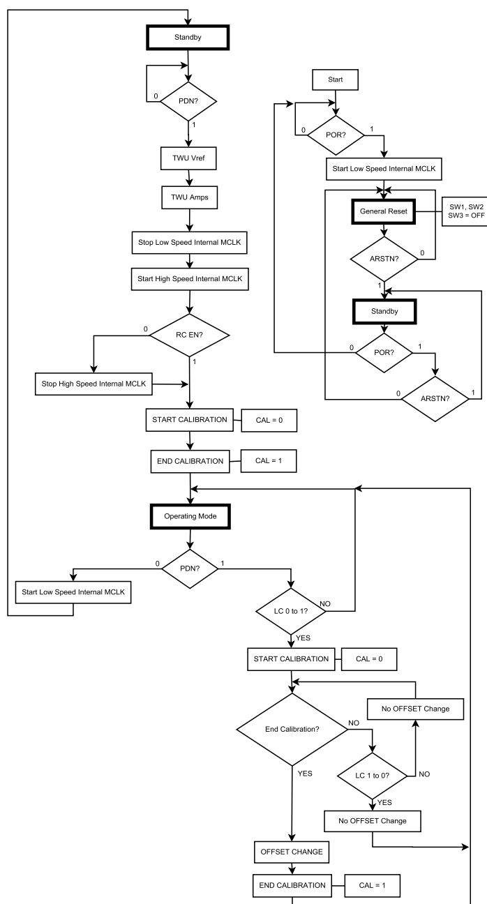
Figure 16. DAC operation flow chart (main)
