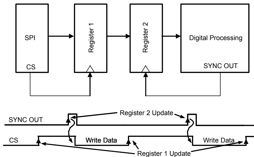
Figure 12. Synchronous DAC data update
