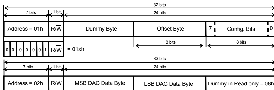
Figure 9. Data and control frame format
