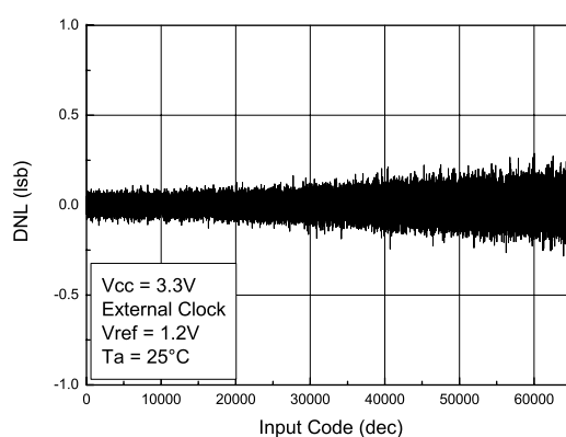
Figure 28. DNL vs. input code, external master clock, AVCC = 3.3 V
