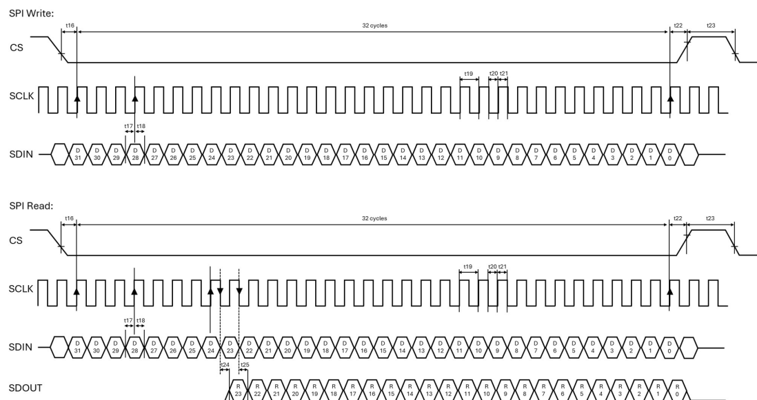
Figure 24. DAC timing diagram 3
