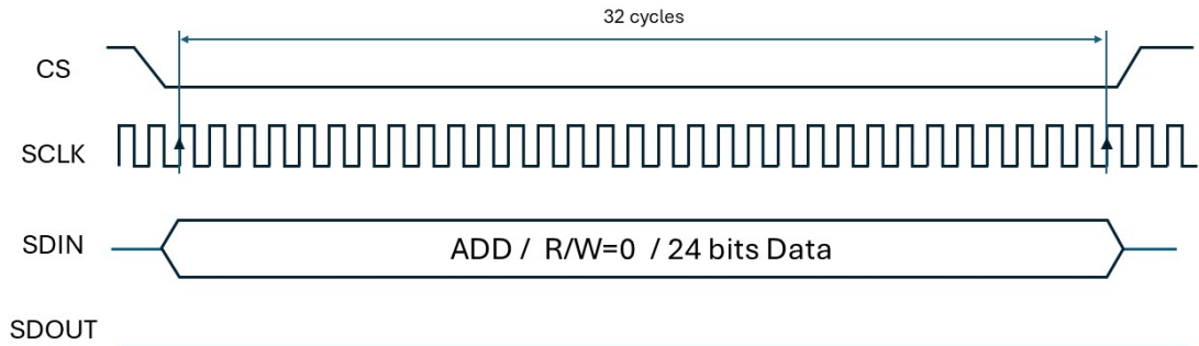
Figure 7. SPI write sequence
