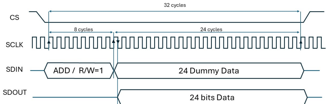
Figure 8. SPI read sequence
