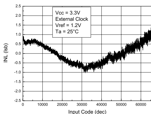
Figure 27. INL vs. input code, external master clock, AVCC = 3.3 V
