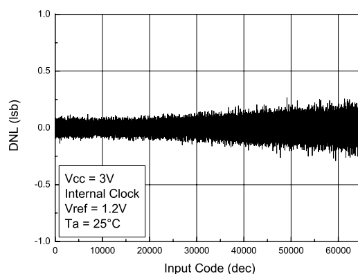
Figure 30. DNL vs. input code, internal master clock, AVCC = 3 V
