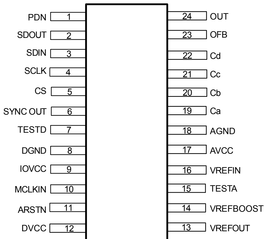
Figure 3. Pin locations
