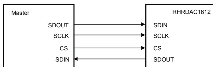
Figure 4. SPI interface connections for stand-alone operations
