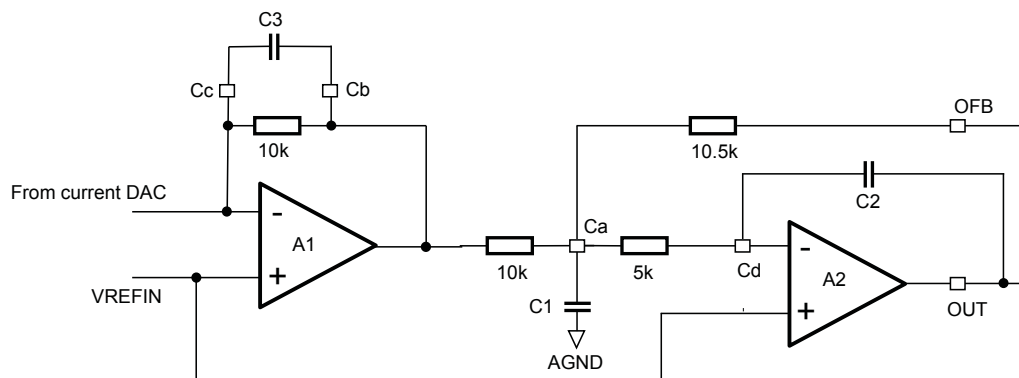
Figure 19. Simplified RHRDAC1612 output stage
