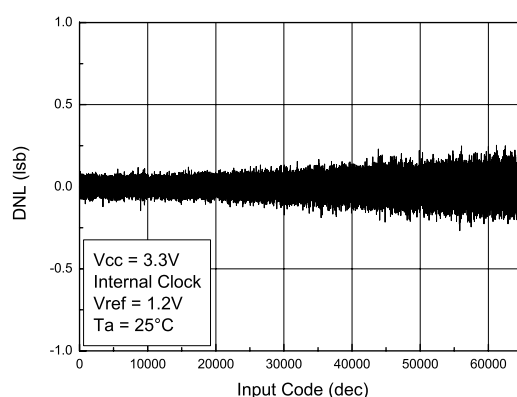
Figure 26. DNL vs. input code, internal master clock, AVCC = 3.3 V
