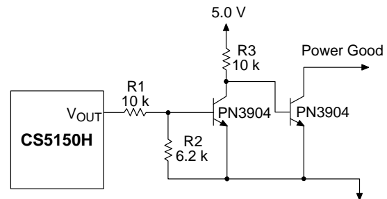
Figure 17. Implementing Power Good with the CS5150H
