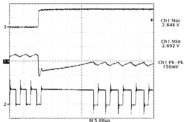
Figure 9. CS5150H Demonstration Board Response to a 0.5 to 13 A Load Pulse (Output Set for 2.8 V)
