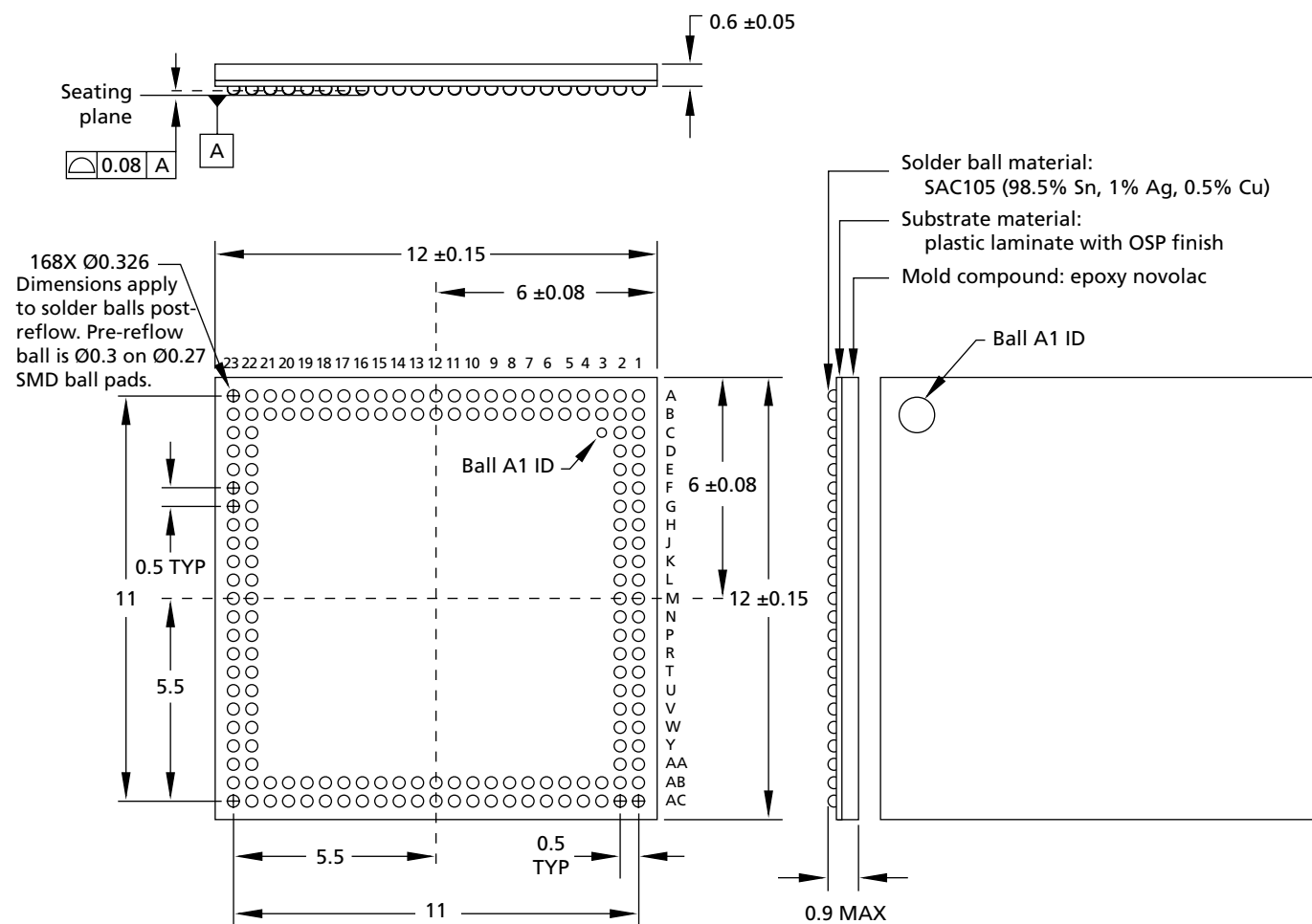
Figure 7: 168-Ball VFBGA
