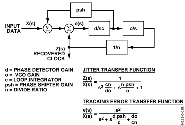
Figure 17. ADN2812 PLL/DLL Architecture
