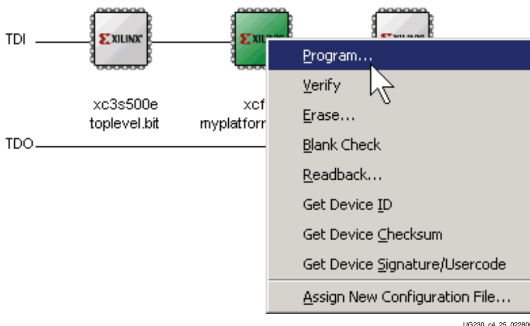
Figure 4-24: Program the XCF04S Platform Flash PROM
