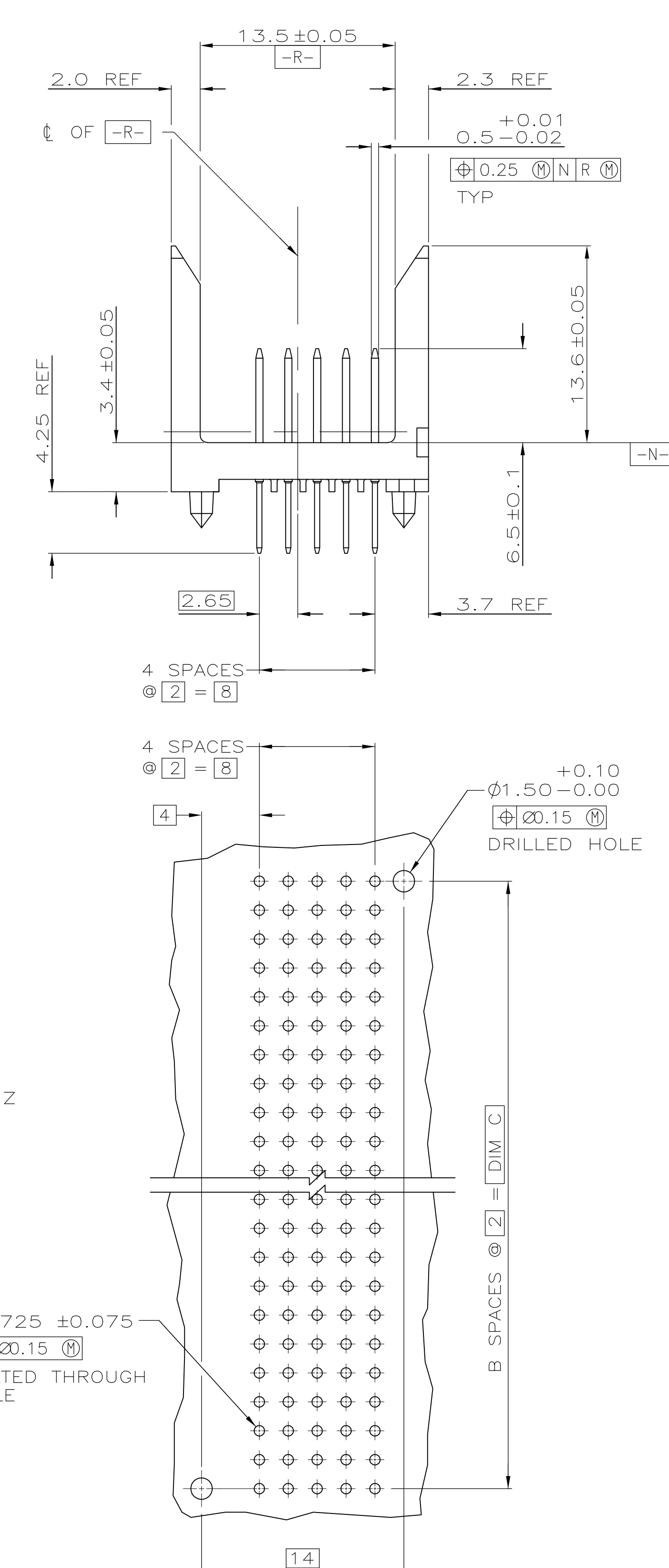
RECOMMENDED CIRCUIT PATTERN (COMPONENT SIDE)
