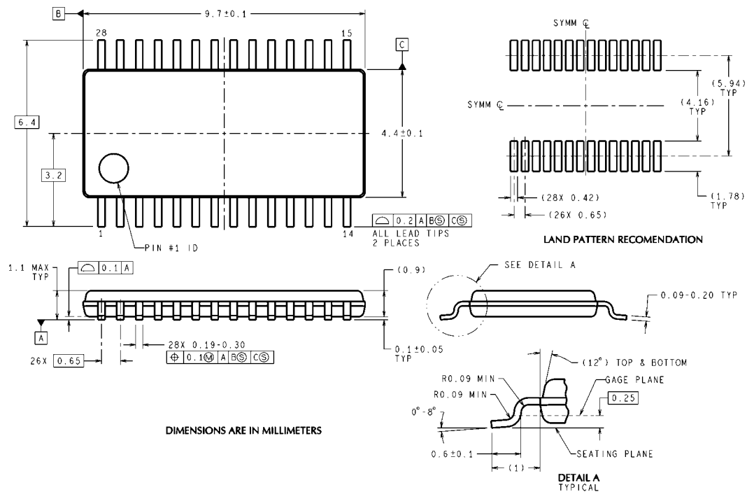
28-Lead TSSOP Package Ordering Number ADC10080CMT NS Package Number MTC28
