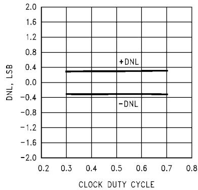
DNL vs. Clock Duty Cycle (DC input)
