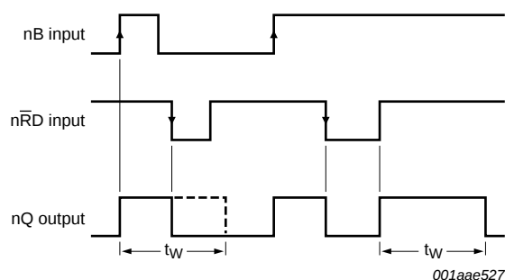
Fig 9. Output pulse control using reset input \overline{nRD}
