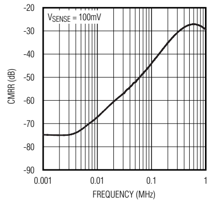
POUT COMMON-MODE REJECTION RATIO vs. FREQUENCY
