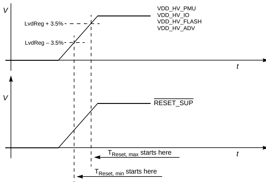
Figure 19. External VREG mode, RESET_SUP rises with V DD_HV_XXX
