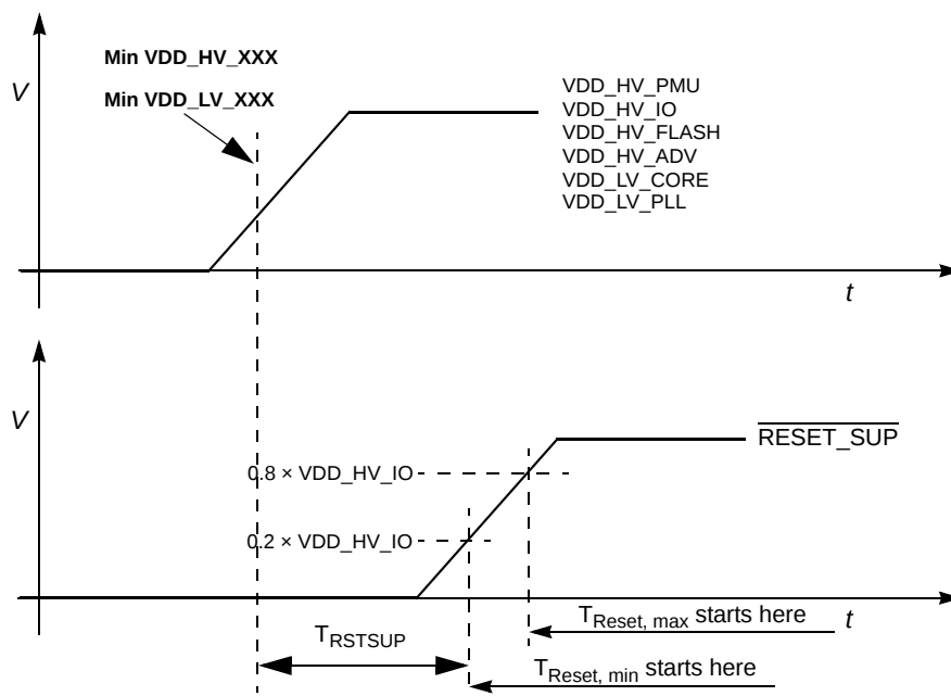
Figure 18. External VREG mode, RESET_SUP rises after V DD_HV_XXX are stable
