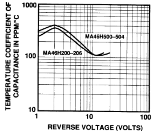
Temperature Coefficient of Capacitance vs Reverse Voltage
