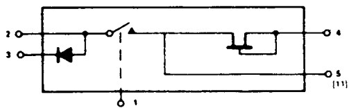
IH5022 (8 LEAD PDIP, 14 LEAD CERNIP)
