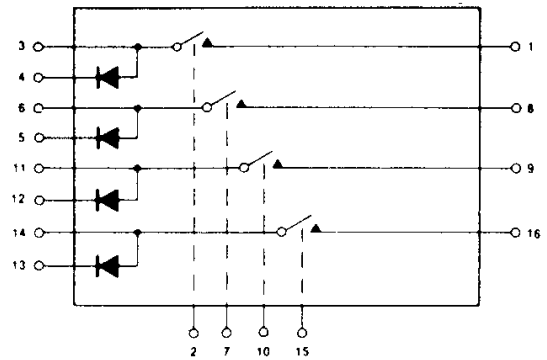
IH5011, IH5012 (16 LEAD CERNIP, 16 LEAD PDIP)
