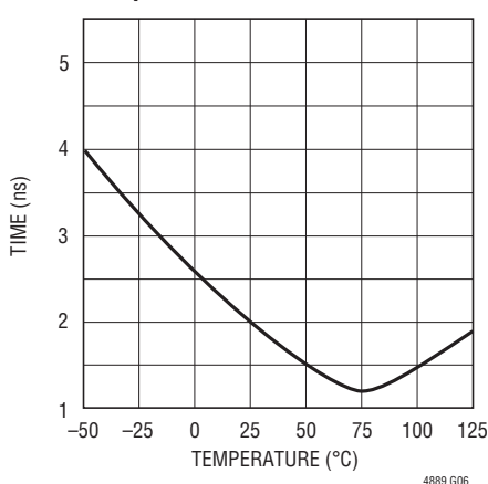
Receiver |t_{PLH} - t_{PLH}| vs Temperature
