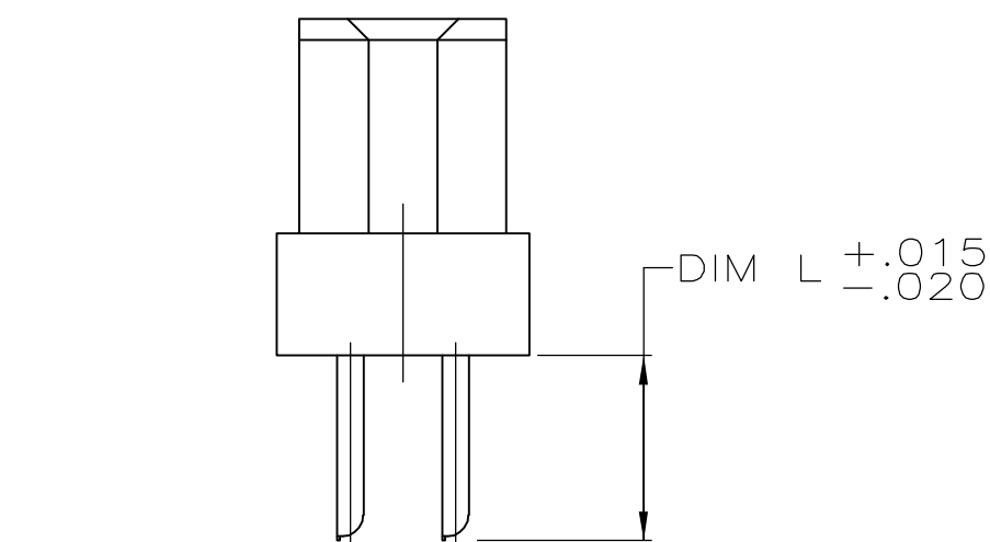
TYPE II SOLDER EYELET CONTACT
