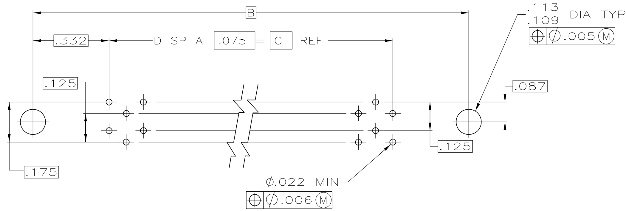
RECOMMENDED P.C. BOARD LAYOUT FOR TYPE I ASSEMBLIES ONLY
