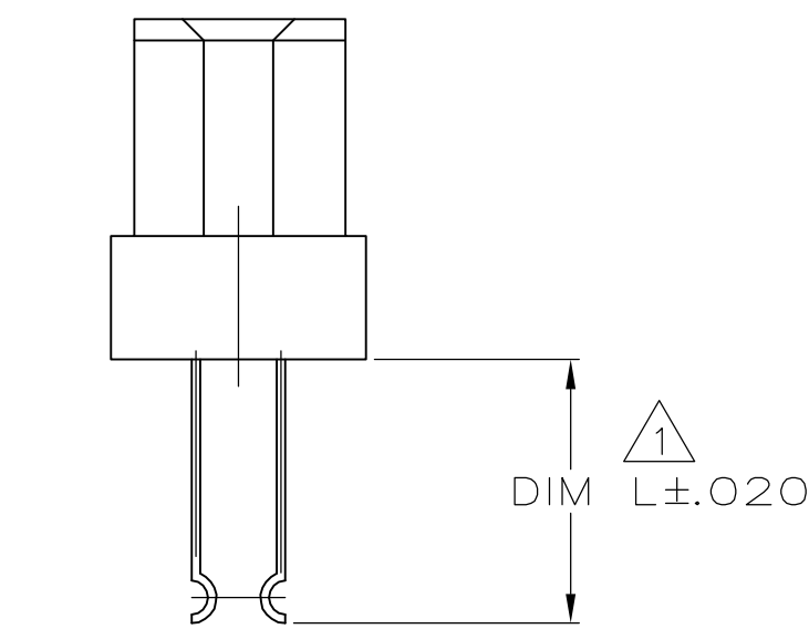
TYPE III CARD EXTENDER TYPE CONTACT
