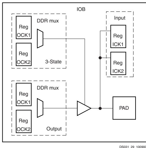
Figure 3: Virtex-II IOB Block
