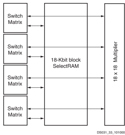
Figure 36: SelectRAM and Multiplier Blocks
