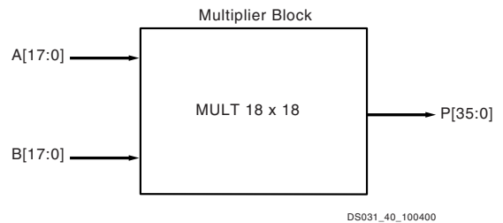
Figure 37: Multiplier Block
