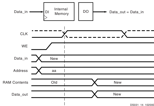
Figure 32: WRITE_FIRST Mode
