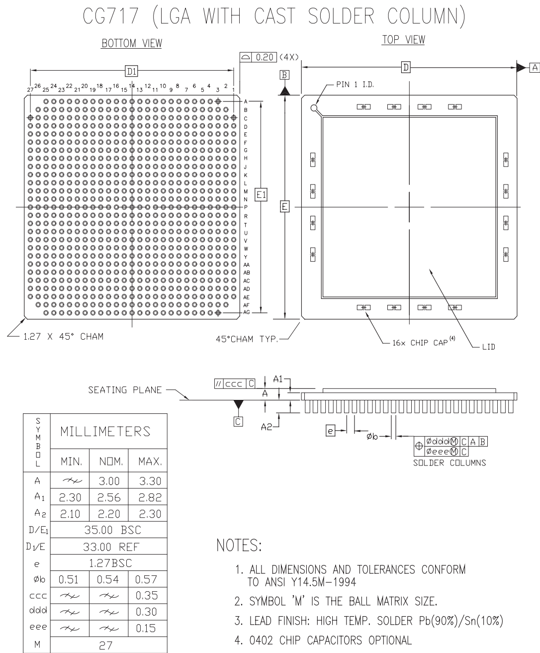
Figure 55: CG717 Ceramic CGA Package Specifications
