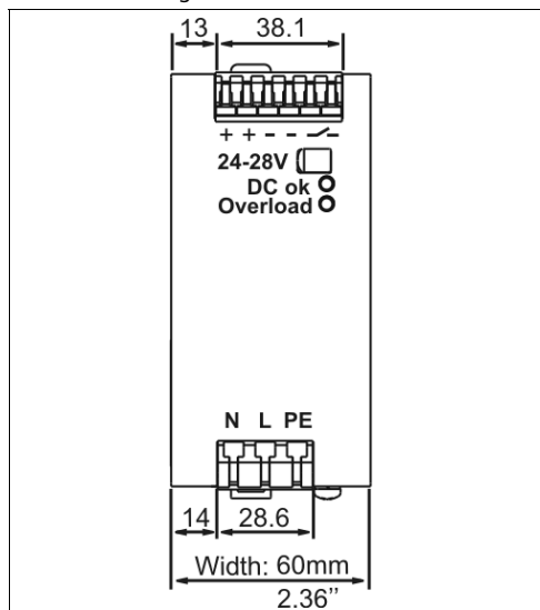
Fig. 22-1 Front view
