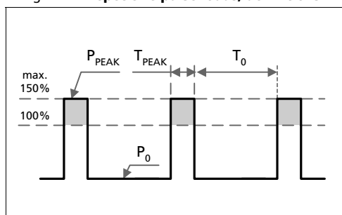
Fig. 24-1 Repetitive pulse loads, definitions
