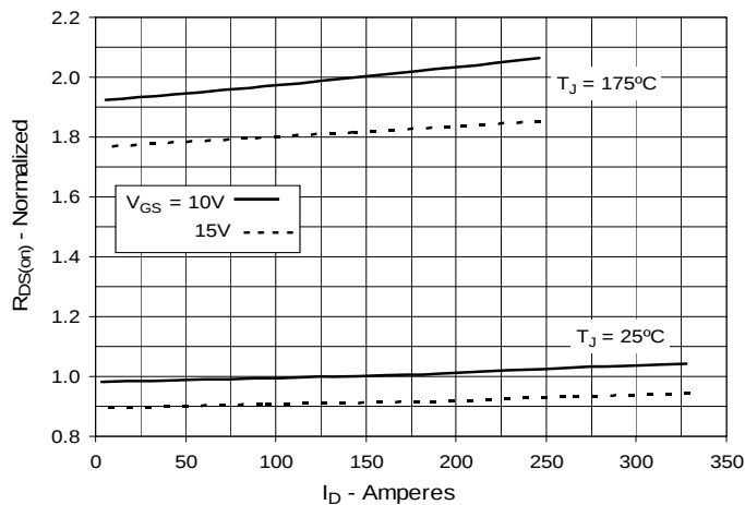
Fig. 5. R_{DS(on)} Normalized to I_D = 140\text{A} Value vs. Drain Current
