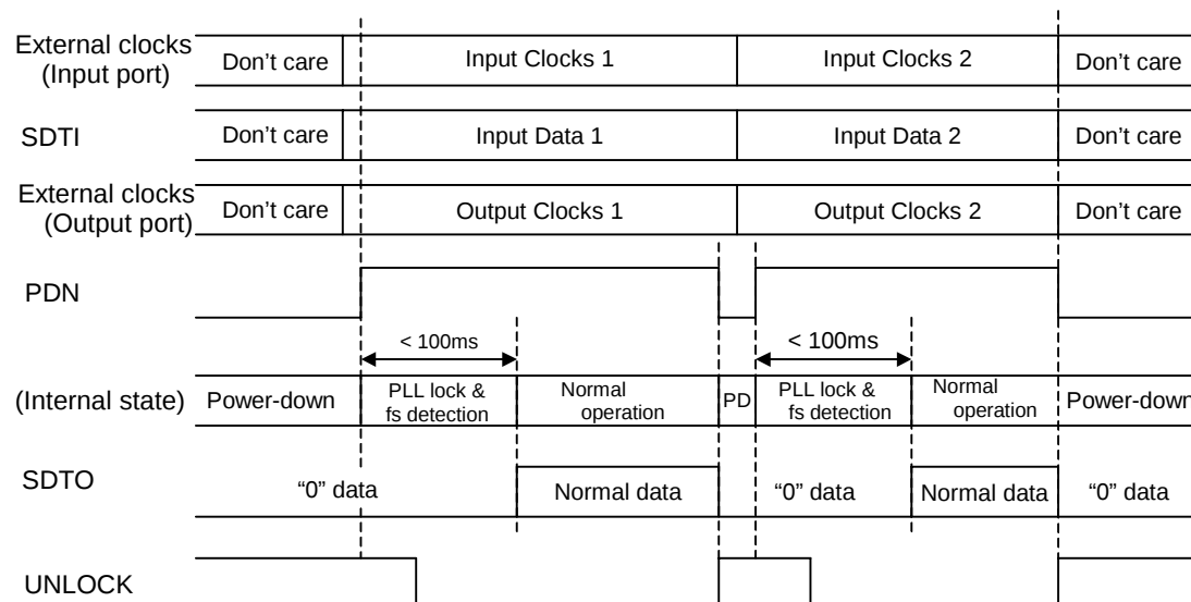
Figure 12. System Reset
