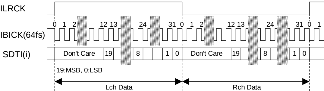
Figure 3. Mode 1 Timing
