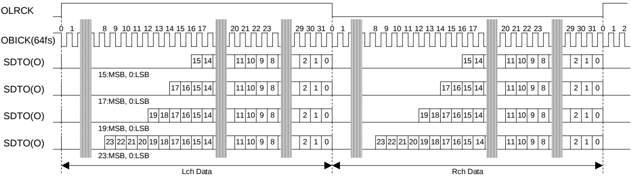
Figure 7. LSB Timing
