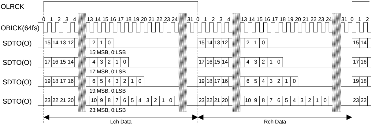
Figure 8. MSB Timing
