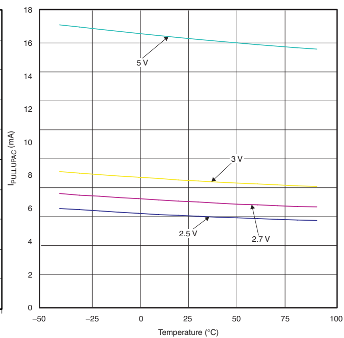
Figure 4. I_{PULLUPAC} vs Temperature
