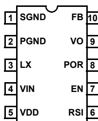
EL7532 (10 LD MSOP) TOP VIEW
