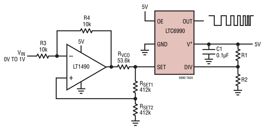
Full Range VCO with Any N_{DIV} Setting (Positive Frequency Control, f_{MIN} to f_{MAX} for V_{IN} = 0V to V_{SET} )
