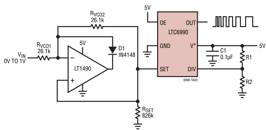
Full Range VCO with Any N_{DIV} Setting ( f_{MAX} to f_{MIN} for V_{IN} = 0V to V_{SET} )
