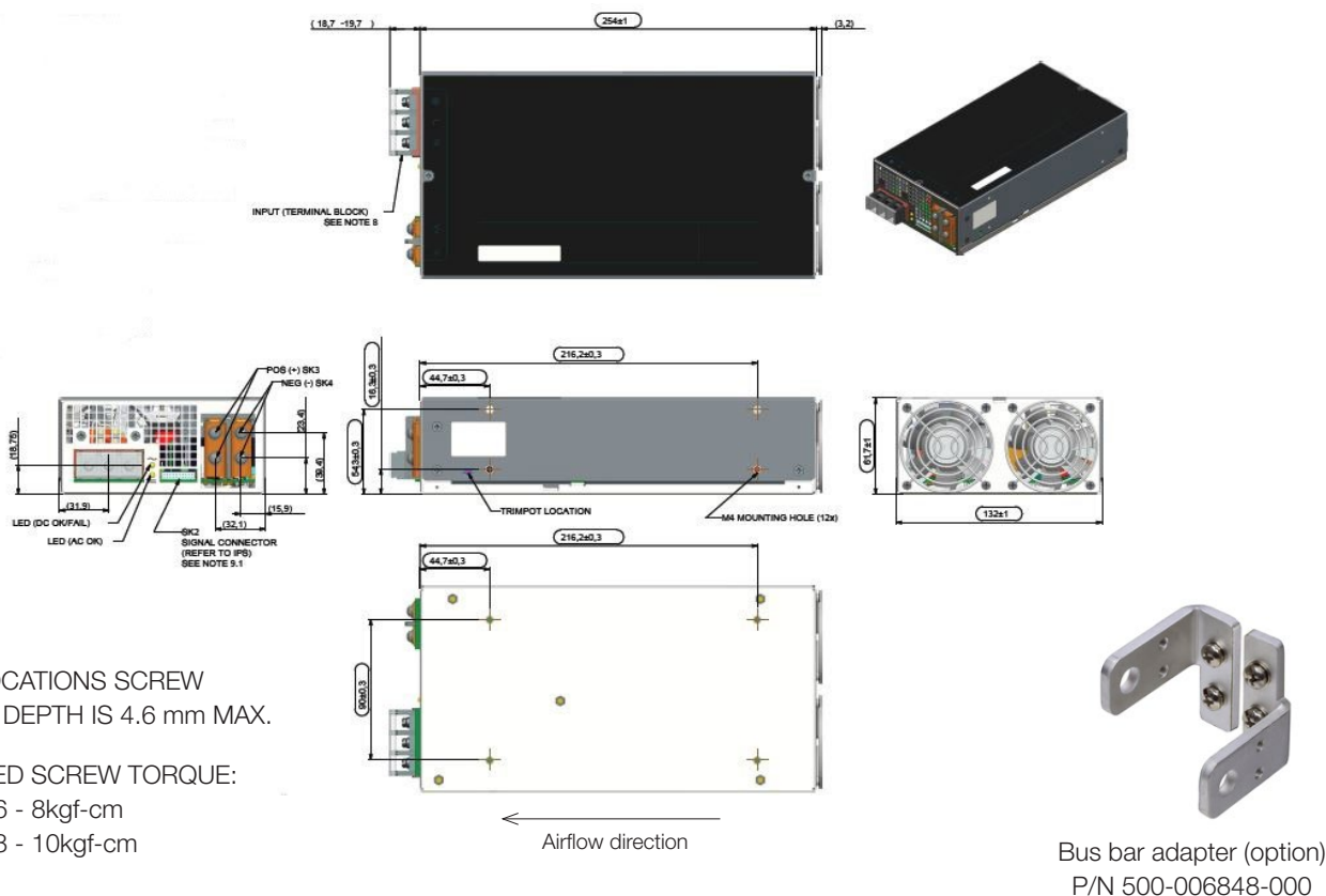
Mechanical Drawings (LCM1000Q-T, LCM1000U-T and LCM1000W-T)
