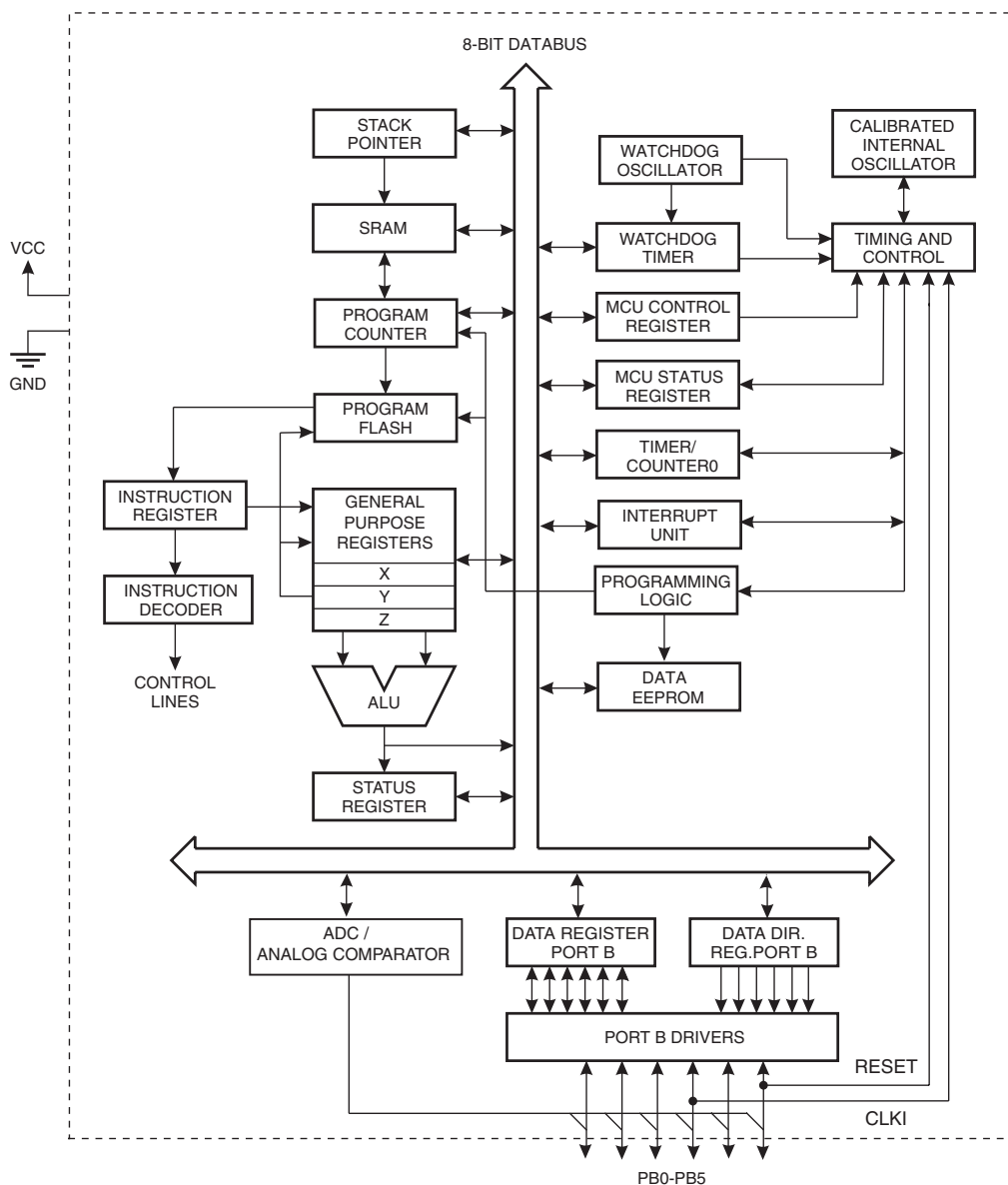
Figure 2. Block Diagram
