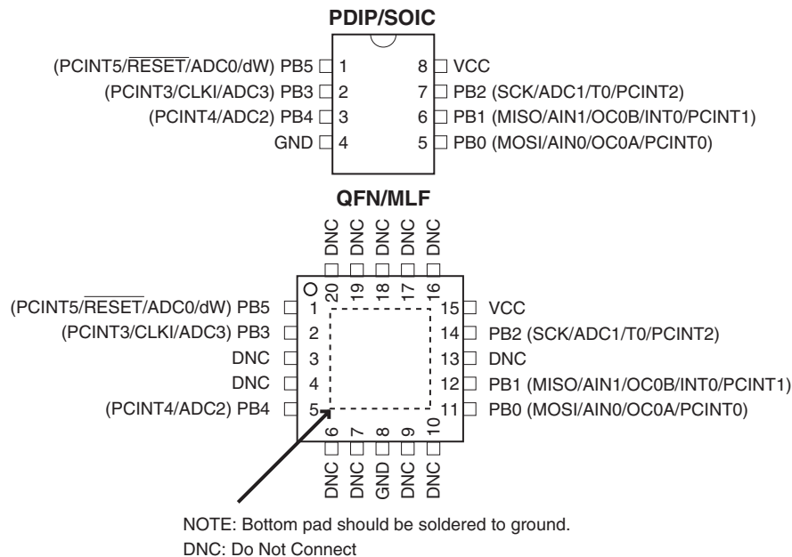
Figure 1. Pinout ATtiny13
