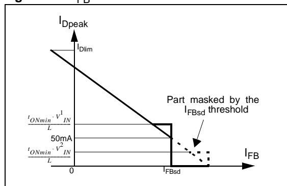
Figure 10 : I_{EB} Transfer function
